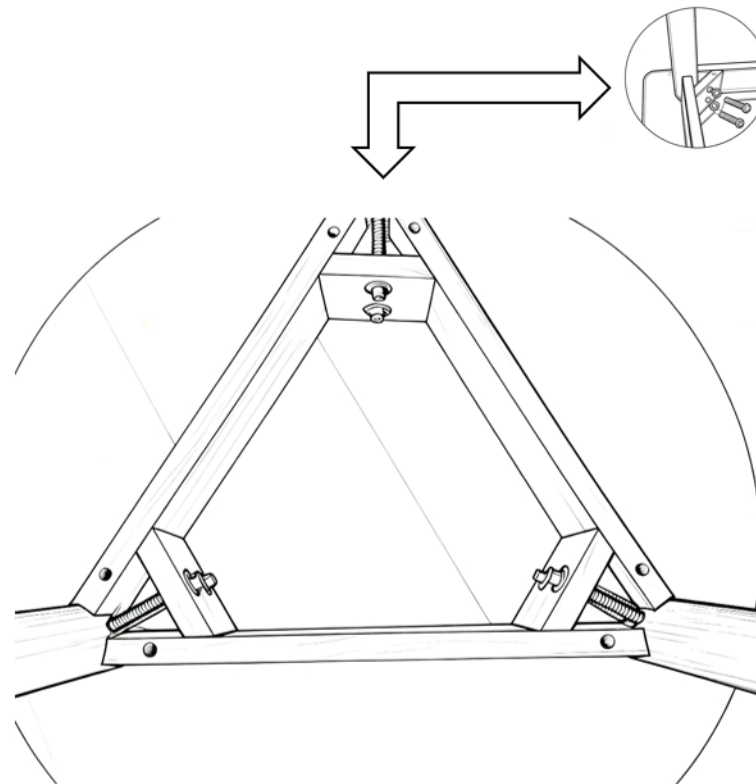
assembly drawing
